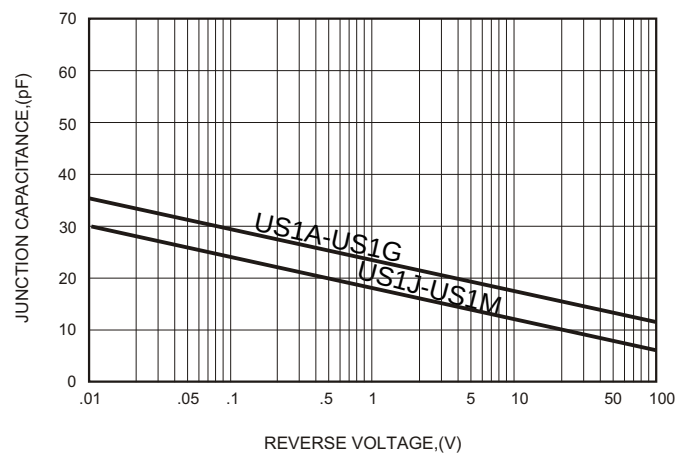
FIG.6-TYPICAL JUNCTION CAPACITANCE
