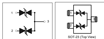
Schematic & PIN Configuration
