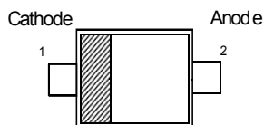
SOD-523
