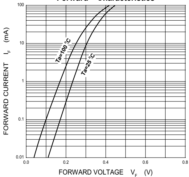
Forward Characteristics
