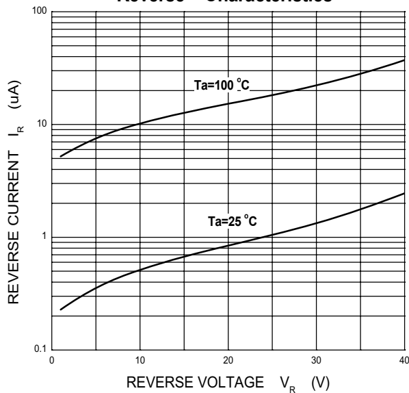
Reverse Characteristics
