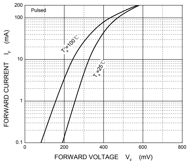
FIG.2-TYPICAL FORWARD CHARACTERISTICS
