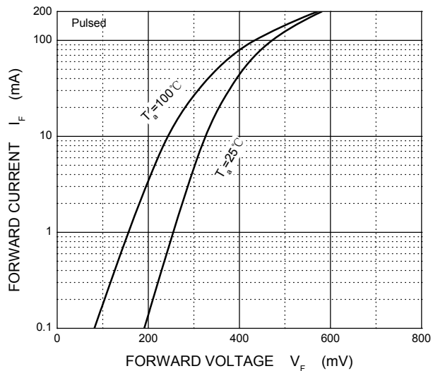
FIG.1-Forward Characteristics
