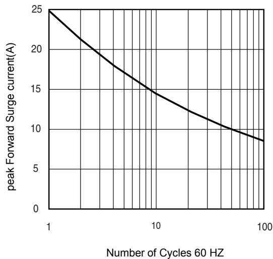
FIG.4-Power Derating Curve
