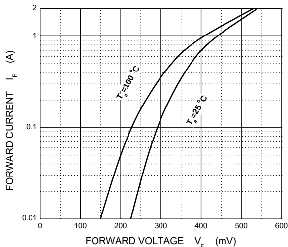
FIG.2-TYPICAL FORWARD CHARACTERISTICS
