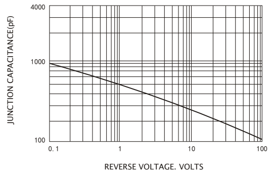
FIG.5-TYPICAL JUNCTION CAPACITANCE
