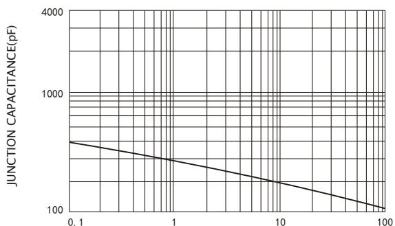
FIG.5-TYPICAL JUNCTION CAPACITANCE
