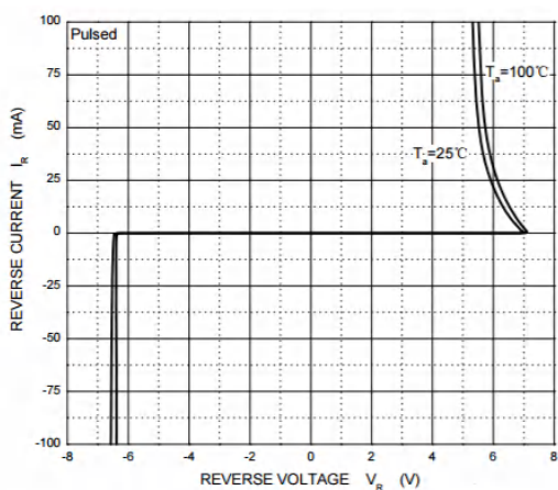
Reverse Characteristics
