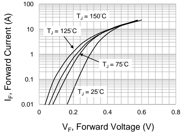
FIG.2-TYPICAL FORWARD CHARACTERISTICS
