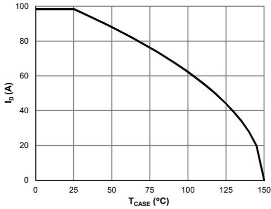
Figure 7: Current De-rating
