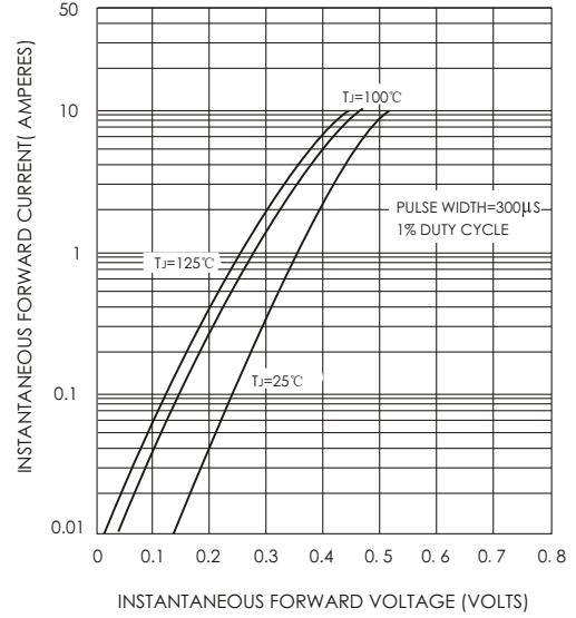
FIG.2-TYPICAL FORWARD CHARACTERISTICS
