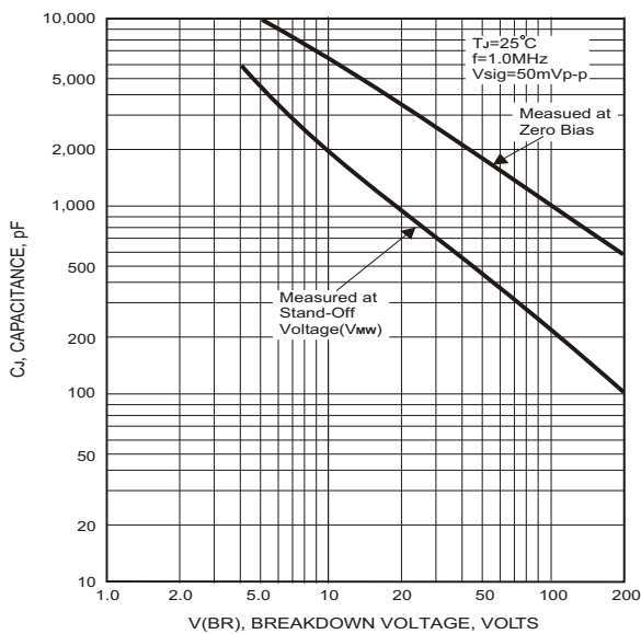
FIG.5-TYPICAL JUNCTION CAPACITANCE
