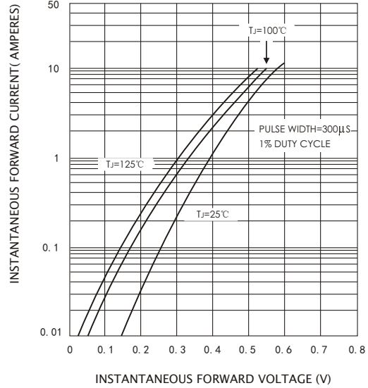
FIG.2-TYPICAL FORWARD CHARACTERISTICS
