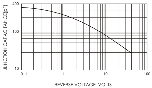
FIG.5-TYPICAL JUNCTION CAPACITANCE
