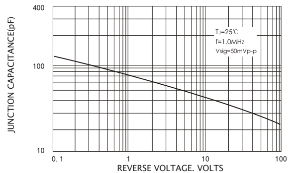
FIG.5-TYPICAL JUNCTION CAPACITANCE
