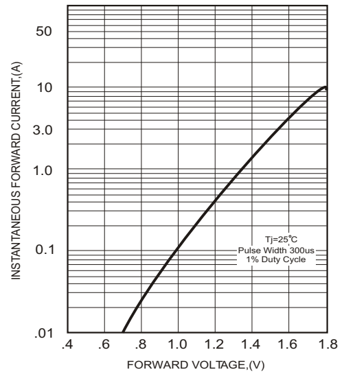
FIG.2-TYPICAL FORWARD CHARACTERISTICS
