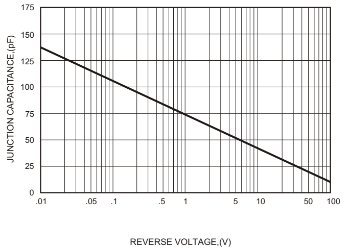
FIG.6-TYPICAL JUNCTION CAPACITANCE
