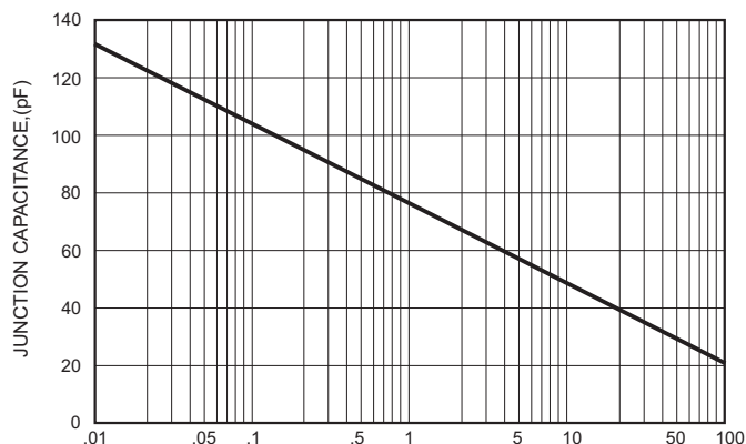
FIG.5-TYPICAL JUNCTION CAPACITANCE
