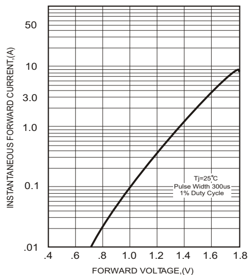
FIG.2-TYPICAL FORWARD CHARACTERISTICS
