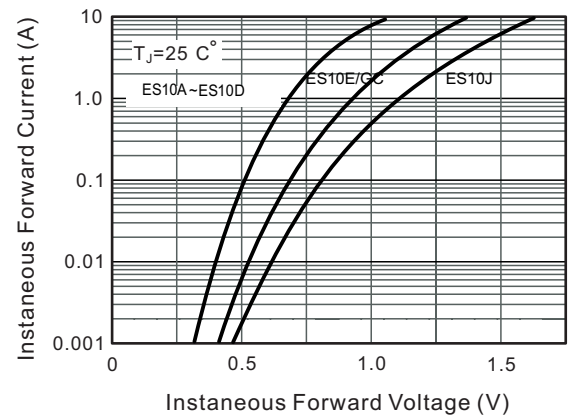
FIG.2-TYPICAL FORWARD CHARACTERISTICS
