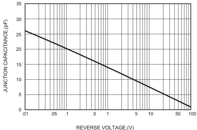
FIG.6-TYPICAL JUNCTION CAPACITANCE
