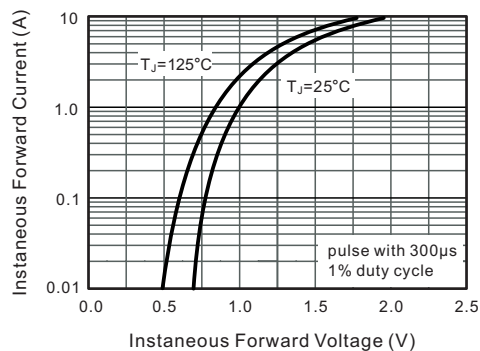
FIG.2-TYPICAL FORWARD CHARACTERISTICS
