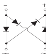
Internal Schematic
